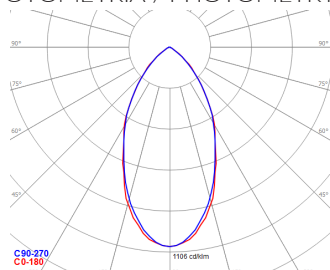
JUDO-3F_55_330W_4000K
